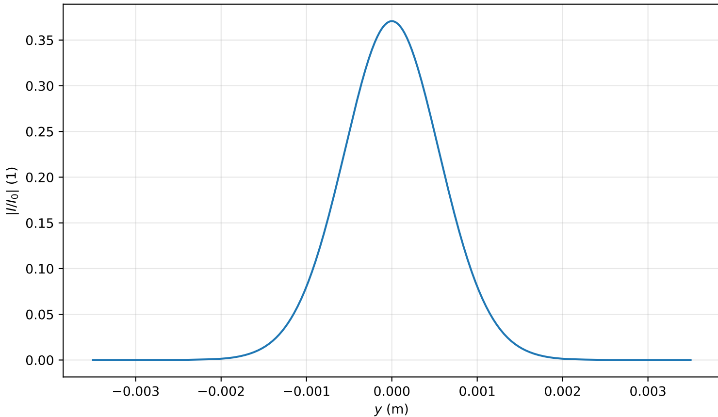
Intensity profile I(x=0, y, z=3.025)/I_0 , P_{in}=0.2P_{cr} , artificial time
